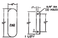
MOUNTING ANGLE & PAD 3 1/2" x 2 1/2" x 1/4" ANGLE W/1/4" PAD (2) EA. REQ'D FOR SECONDARY SHUTOFF MNTG (SHIP LOOSE)
