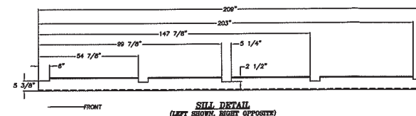
SILL DETAIL (LEFT SHOWN, RIGHT OPPOSITE)
