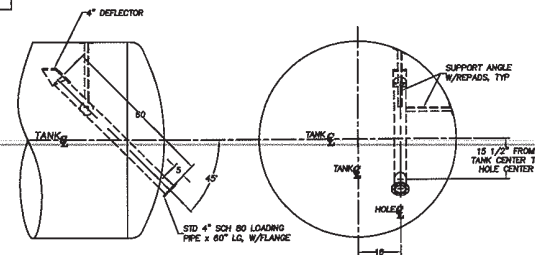
4" REAR LOAD PIPE
