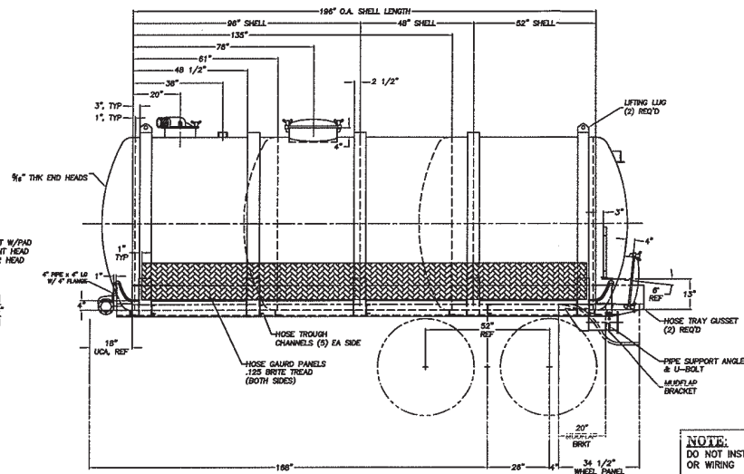
STREET SIDE ELEVATION
