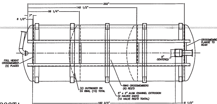
183 3/4 BOTTOM VIEW
